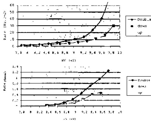
Figure 3.6: Left: intrinsic noise rate in a non oiled RPC. Right: intrinsic noise rate in an oiled RPC (in \text{Hz}/\text{cm}^2 ). In both cases single gap and double gap noise levels are reported. The working point of the detector was at \text{HV} = 9.5 \text{ kV} .
