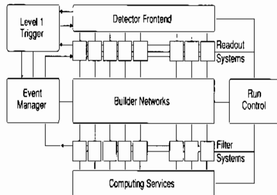
Figure 2.1: CMS Trigger and Data Acquisition System.
