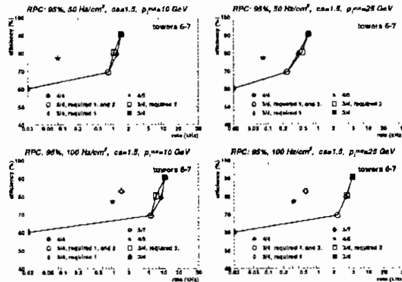
Figure 5.7: Trigger performance in towers 6-7 for various options.
