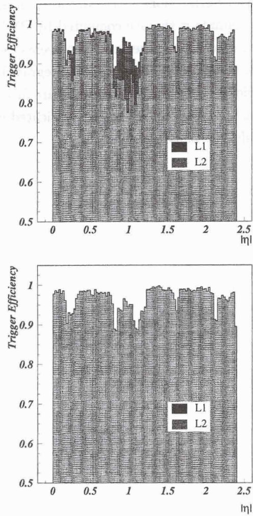
Figure 6.1: L1 and L2 muon reconstruction efficiency as a function of the \eta of the muon at generation. In the left plot RPC information is not included at L2. In the right plot RPC information is included at L2.
