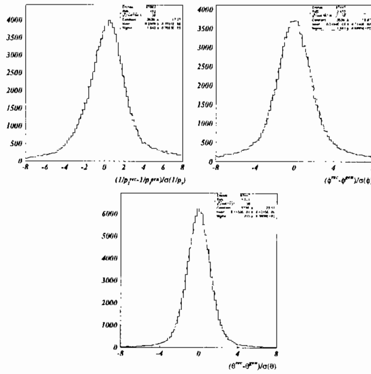
Figure 6.7: L2 pull distributions for the variables 1/p_t (left), \varphi (middle) and \theta (right).
