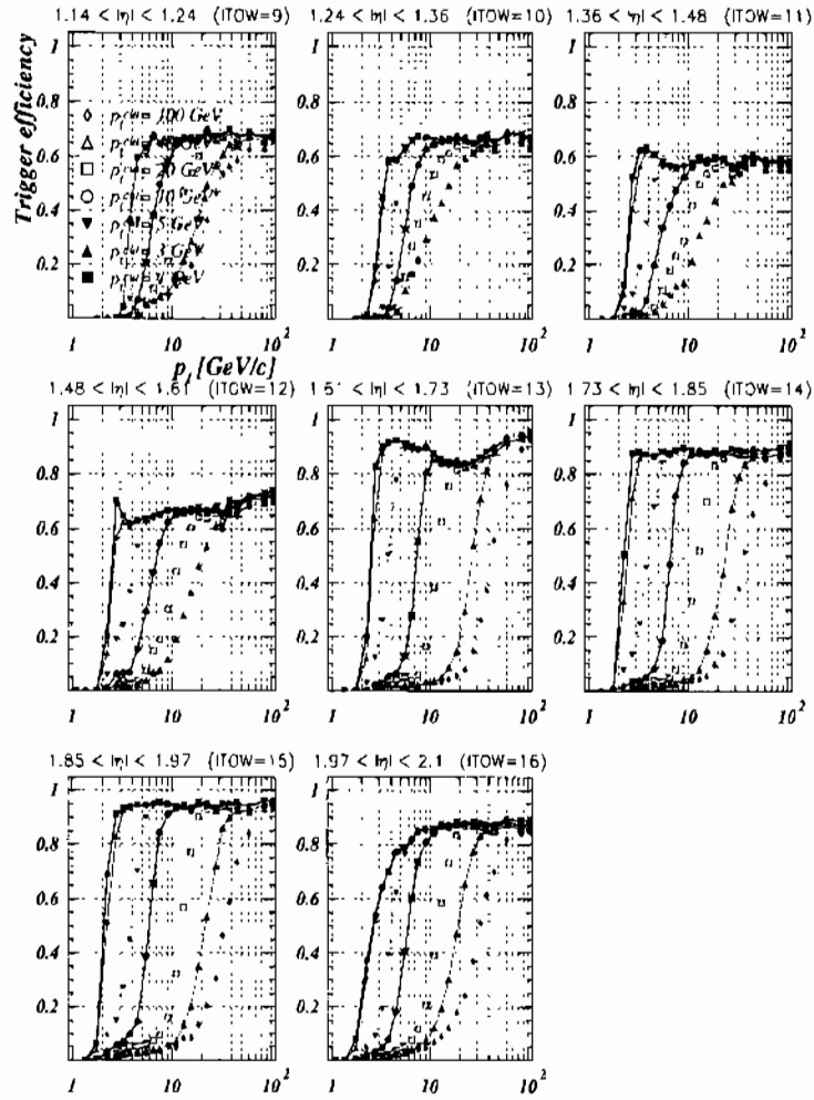
Figure 4.5: Turn-on efficiency curves in towers 9-16 of the RPC system relative to some representative values of the p_t^{cut} as reported on the first plot. The values of the parameters are the following: \epsilon_{RPC} = 0.95 , \sigma_{RPC} = 2.5 ns, cs = 1.5 strips noise_{RPC} = 50 Hz cm^{-2} , ratefac = 1 , gatewidth = 20 \mu s . Only 4 out of 4 coincidences are allowed in towers 9-12.
