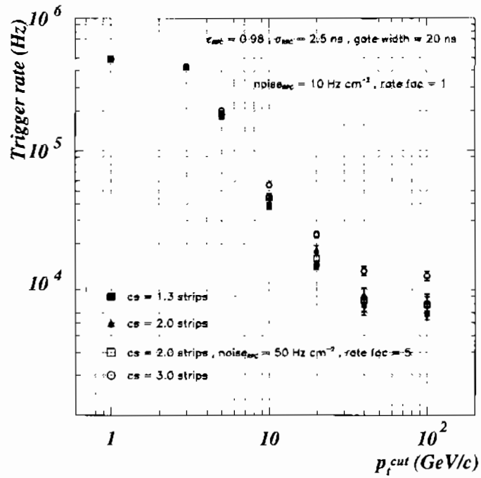
Figure 4.14: Decay muons trigger rate versus p_t^{cut} at L = 10^{34} cm^{-2}s^{-1} . Various scenarios from the point of view of cluster size and noise and background hit rates are considered as reported on the plot. The contribution from pure coincidences of noise and background hits has been subtracted out as described in the text.
