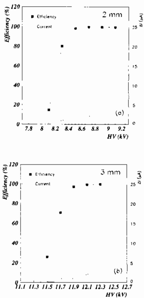
Figure 3.8: Average efficiency and current versus HV for the 2 mm (a) and 3 mm (b) chamber in the central 10 \times 10 \text{ cm}^2 trigger region. Fluctuations around the average are also shown.
