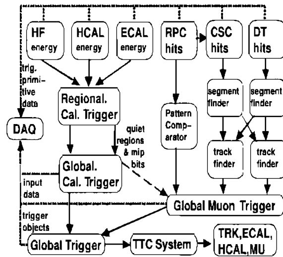
Figure 2.2: Overview of the CMS Level 1 Trigger.
