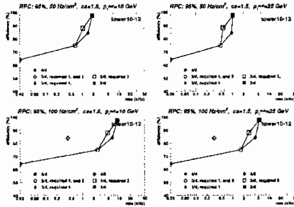
Figure 5.10: Trigger performance in towers 10-12 for various options.
