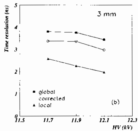
Figure 3.17: Time resolution versus HV for the 2 mm (a) and 3 mm (b) chamber.
