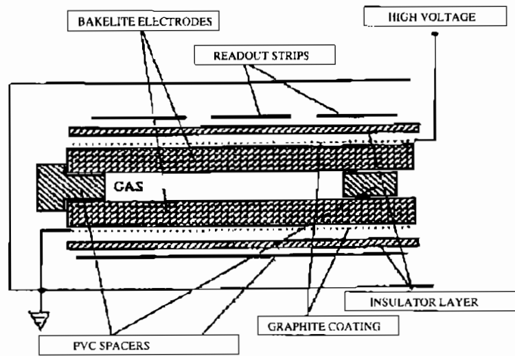
Figure 3.1: Schematic view of a single gap RPC.
