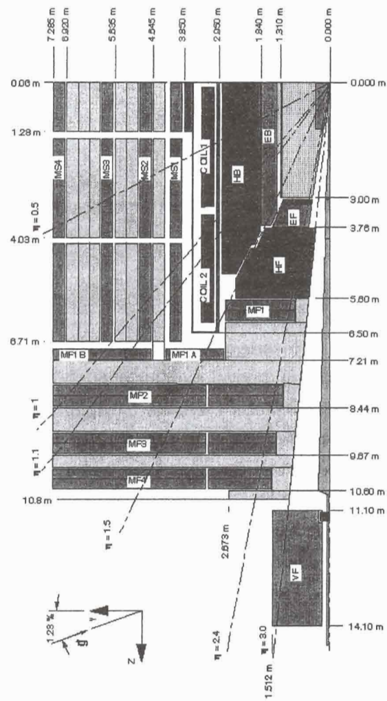
Figure 1.19: Longitudinal view of the CMS detector.
