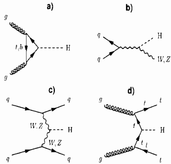
Figure 1.5: Tree level Feynman diagrams contributing to the Higgs production in hadron collisions.
