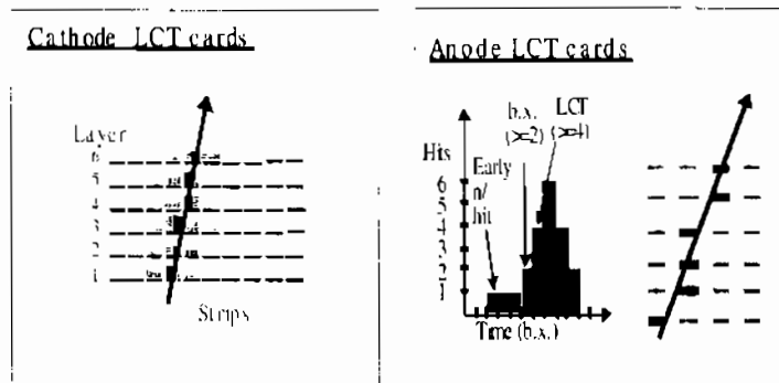
Figure 2.5: Principle of the CSC Local Trigger.
