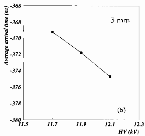
Figure 3.18: Average arrival time (arbitrary zero) versus HV for the 2 mm (a) and 3 mm (b) chamber.
