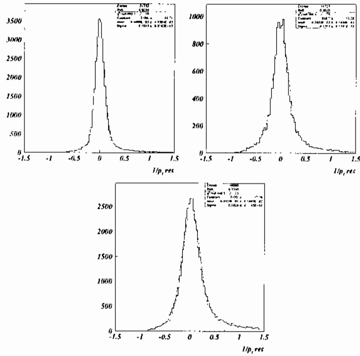
Figure 6.3: 1/p_t resolution at L2 without use of RPC information. The variable (1/p_t^{rec} - 1/p_t^{gen})/1/p_t^{gen} is plotted separately in the barrel ( |\eta| < 0.8 , left), overlap ( 0.8 < |\eta| < 1.2 , middle) and endcap ( 1.2 < |\eta| < 2.4 , right).
