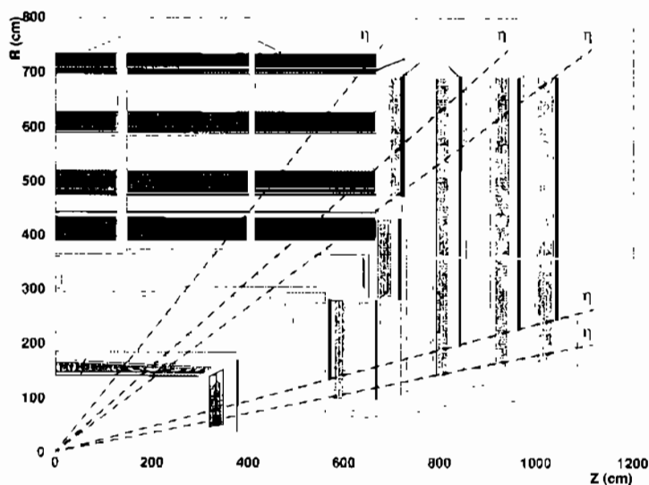
Figure 1.21: The CMS muon detectors.
