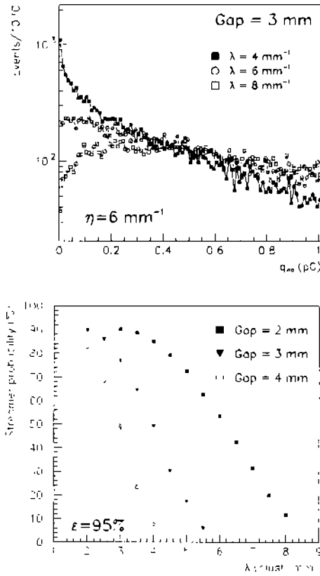
Figure 3.4: Left: simulated charge spectra for three different \lambda values. Right: streamer probability as a function of \lambda for three different gap widths.
