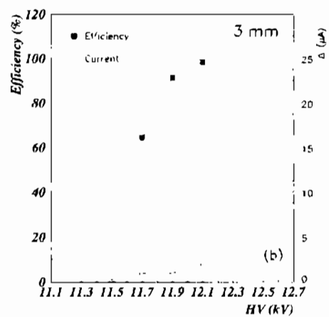
Figure 3.12: Efficiency versus HV for the 2 mm (a) and the 3 mm (b) chamber, computed as the average over 1600 cells.
