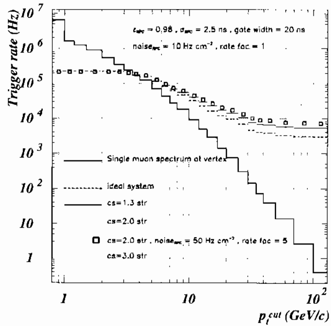
Figure 4.8: RPC single muon trigger rate due to prompt muons versus p_t^{cut} for L = 10^{34} \text{cm}^{-2}\text{s}^{-1} . Various scenarios from the point of view of cluster size, noise and background hit rates are considered as reported on the plot.
