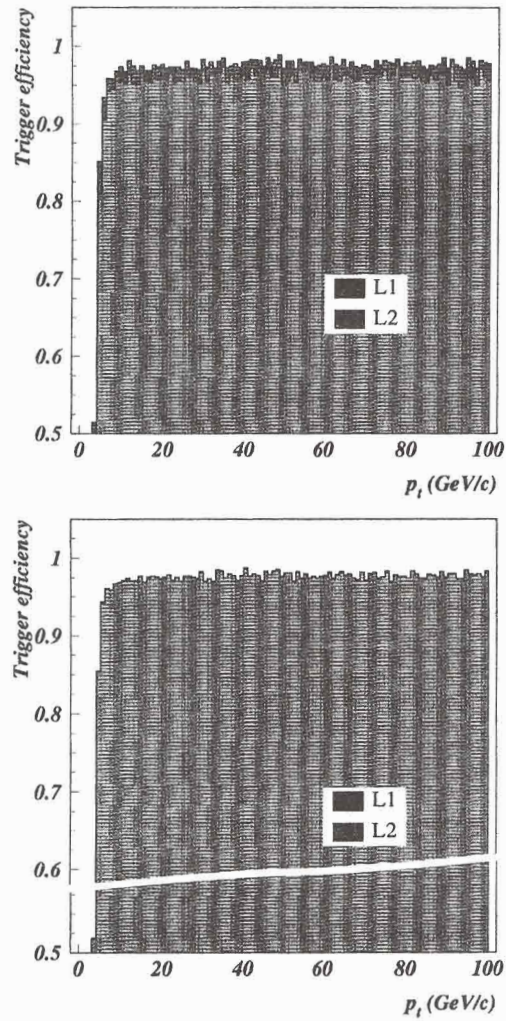
Figure 6.2: L1 and L2 reconstruction efficiency as a function of the muon p_t at generation. In the left plot RPC information is not included at L2. In the right plot RPC information is included at L2.
