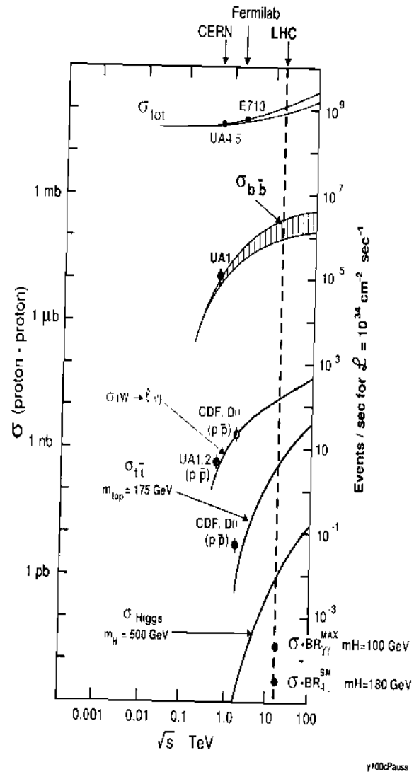
Figure 1.3: Cross sections in proton-proton collisions as a function of the center of mass energy [18].
