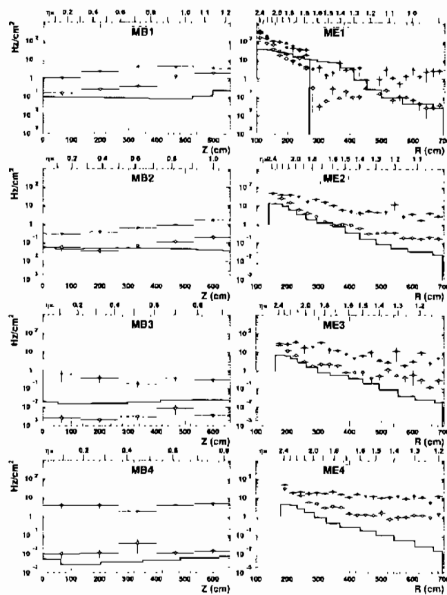
Figure 1.22: Hit rates expected in the CMS muon chambers at 10^{34} \text{ cm}^{-2}\text{s}^{-1} . Full lines indicate the hit rate due to real muons. Empty circles refer to punch-through hadrons, whereas full circles correspond to hits caused by neutral particles background.
