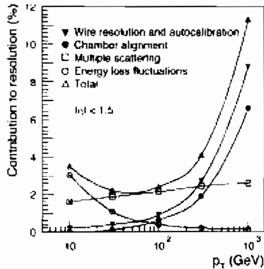
Figure 1.16: The various momentum contribution to the momentum resolution for muons in the ATLAS detector.
