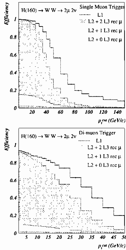
Figure 6.16: Single (left) and di-muon (right) trigger efficiency as a function of p_t^{cut} for the channel H(160 \text{ GeV}/c^2) \rightarrow W^+W^- \rightarrow \mu^+\mu^-\nu_\mu\bar{\nu}_\mu . The fraction of events passing L2 is further divided according to the number of signal muons that are successfully reconstructed at L3. The sample is subject to the kinematical cuts described in the text.
