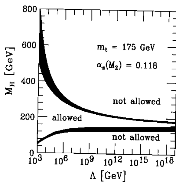
Figure 1.1: The lower and upper Higgs mass theoretical bounds as a function of the energy scale \Lambda at which the Standard Model breaks down. The shaded areas reflect the theoretical uncertainties in the calculation of the Higgs mass bound [6]
