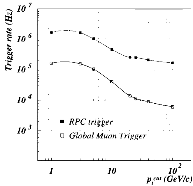
Figure 5.1: RPC false trigger rate as a function of p_t^{cut} . The rate accepted by the GMT adopting its standard selection algorithm is also shown.
