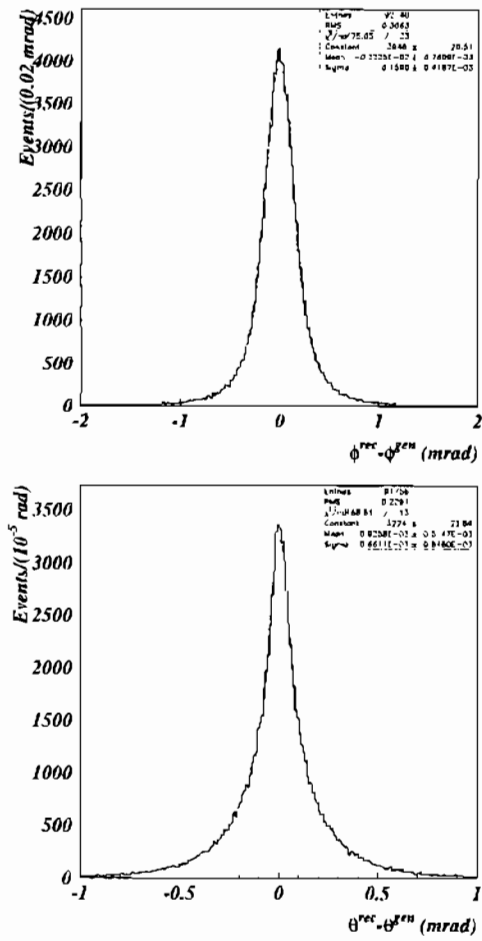
Figure 6.12: L3 \varphi (left) and \theta (right) residual distribution.
