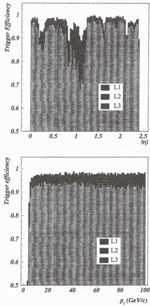
Figure 6.10: L3, L2 and L1 muon reconstruction efficiency as a function of the muon \eta (left) and p_t (right) at generation.
