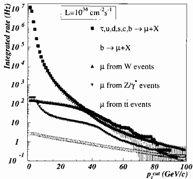
Figure 1.13: Single muon integrated rate at generation level (PYTHIA 6.152) as a function of p_t^{\text{cut}} . The different dominant sources are shown in the plot.
