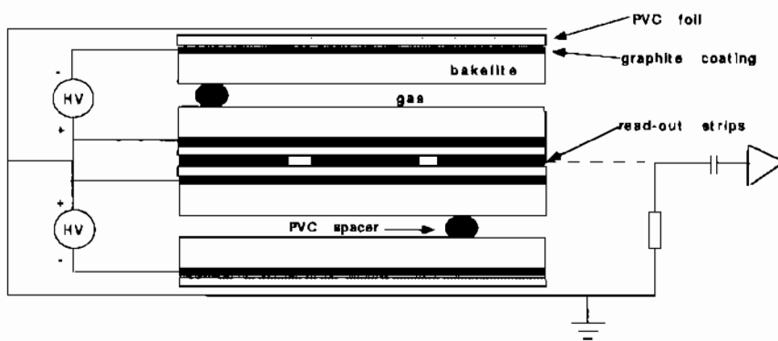
Figure 1.28: Schematic view of a double-gap RPC detector.
