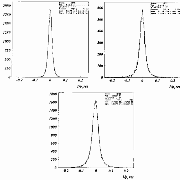
Figure 6.11: L3 1/p_t resolution. The variable (1/p_t^{rec} - 1/p_t^{gen})/1/p_t^{gen} is plotted separately for the barrel ( |\eta| < 0.8 , left), overlap ( 0.8 < |\eta| < 1.2 , middle) and endcap ( 1.2 < |\eta| < 2.4 , right). The corresponding values of the sigmas of the Gaussian fits are: 1.3%, 1.9% and 2.1%.
