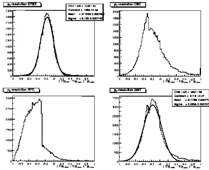
Figure 2.9: 1/p_t resolutions for all systems.
