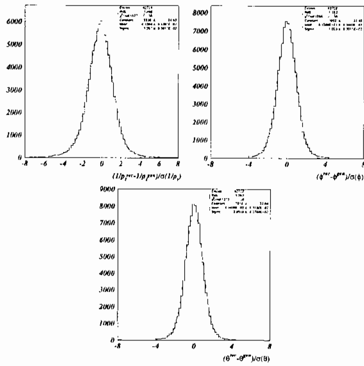
Figure 6.13: L3 pull distributions for the variables 1/p_t (left), \varphi (middle) and \theta (right).
