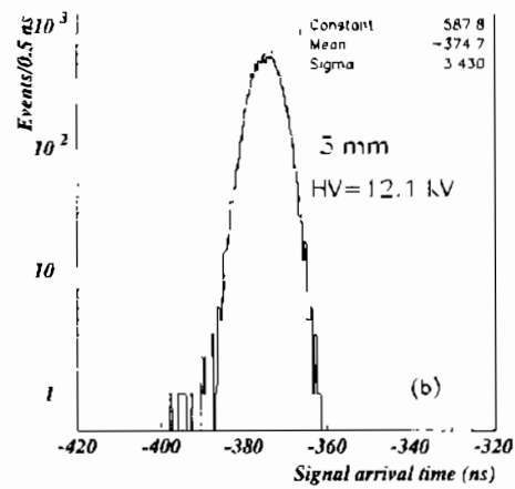
Figure 3.13: Signal arrival time distribution (arbitrary zero) for the 2 mm (a) and the 3 mm (b) chamber.
