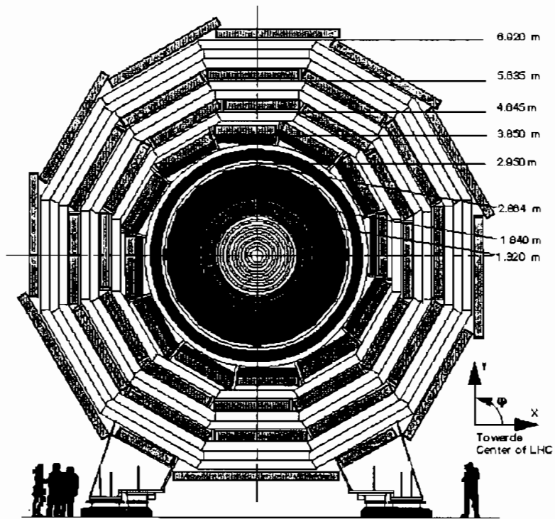
Figure 1.18: Transverse view of the CMS detector.
