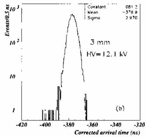
Figure 3.14: Corrected signal arrival time distributions (arbitrary zero) for the 2 mm (a) and the 3 mm (b) chamber.
