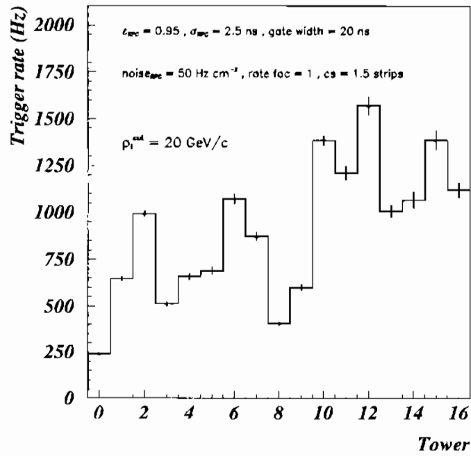
Figure 4.9: RPC single muon trigger rate due to prompt muons versus tower for p_t^{\text{cut}} = 20 \text{ GeV}/c and L = 10^{34} \text{ cm}^{-2}\text{s}^{-1} .
