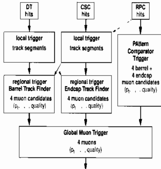
Figure 2.3: Muon Trigger data flow.
