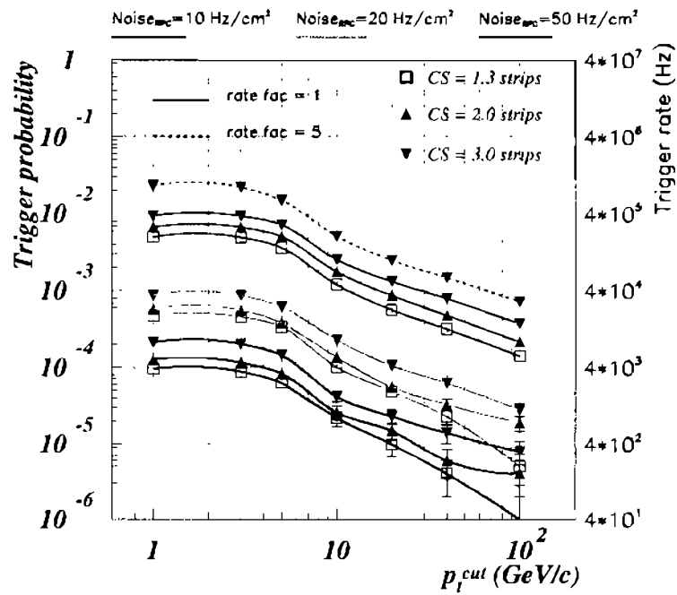
Figure 4.11: RPC false single muon trigger rate due to coincidences of noise and background hits versus p_t^{cut} for various combination of \text{noise}_{RPC} , \text{rate fac} and cs . The rates are calculated for \epsilon_{RPC} = 0.98 , \sigma_{RPC} = 2.5 \text{ ns} and \text{gate width} = 20 \text{ ns} . In towers 9-12 only 4 out 4 coincidences are accepted.
