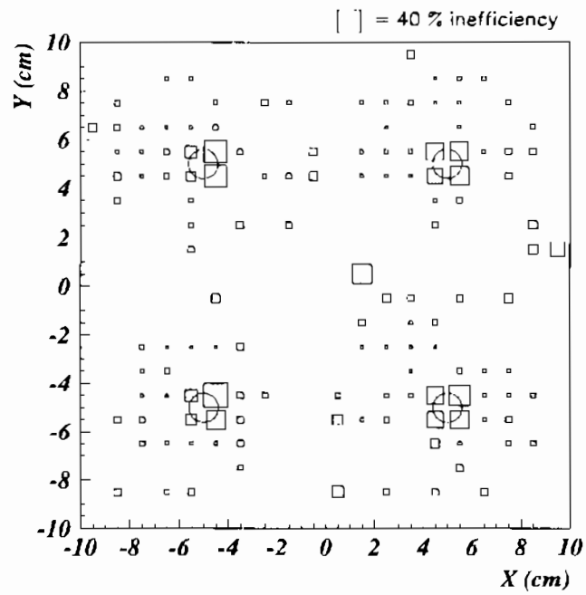
Figure 3.9: Inefficiency map (2 mm, HV=8.9 kV) in the central 20 \times 20 \text{ cm}^2 area of the chamber (circles represent the spacers).
