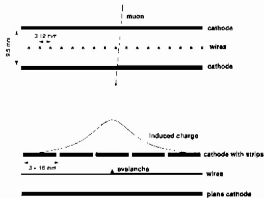
Figure 1.27: Principle of coordinate measurement with a cathode strip chamber: cross-section across wires (top) and across cathode strips (bottom). Close wire spacing allows for fast chamber response, while a track coordinate along the wires can be measured by interpolating strip charges.
