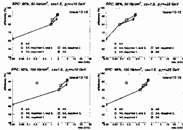
Figure 5.12: Trigger performance in tower 13-16 for various options.
