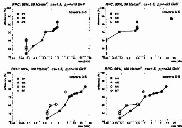
Figure 5.6: Trigger performance in towers 0-5 for various options.
