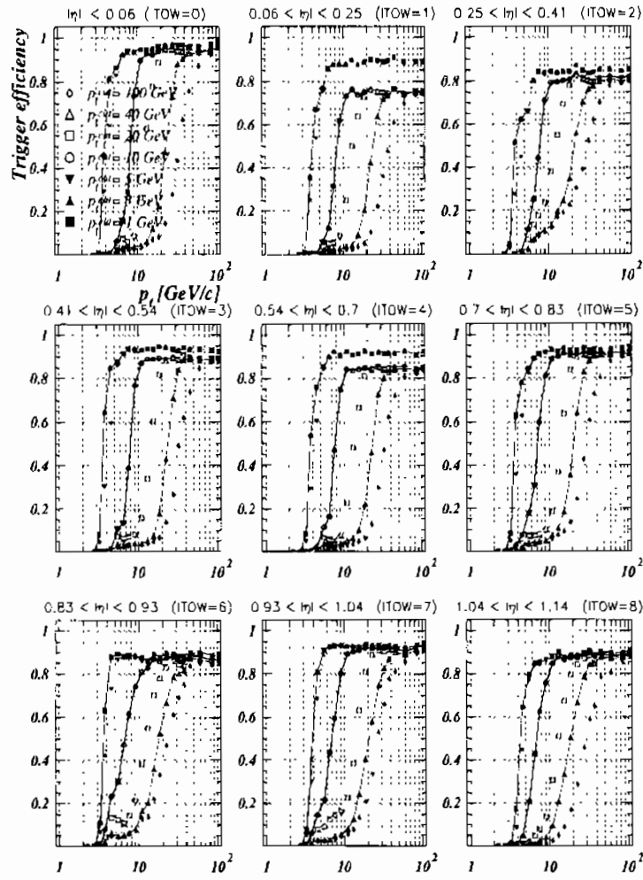
Figure 4.4: Turn-on efficiency curves in towers 0-8 of the RPC system relative to some representative values of the p_t^{cut} as reported on the first plot. The values of the parameters are the following: \epsilon_{RPC} = 0.95 , \sigma_{RPC} = 2.5 ns, cs = 1.5 strips noise_{RPC} = 50 Hz cm^{-2} , ratefac = 1 , gatewidth = 20 ns.
