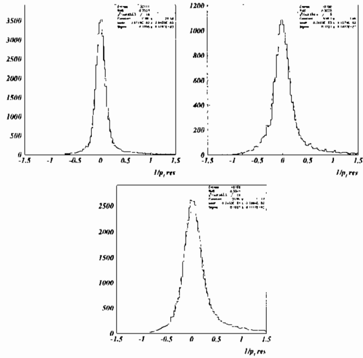
Figure 6.4: 1/p_t resolution at L2 with use of RPC information. The variable (1/p_t^{rec} - 1/p_t^{gen})/1/p_t^{gen} is plotted separately in the barrel ( |\eta| < 0.8 , left), overlap ( 0.8 < |\eta| < 1.2 , middle) and endcap ( 1.2 < |\eta| < 2.4 , right). The corresponding values of the sigmas of the Gaussian fits are: 10.5%, 17.2% and 19.3%
