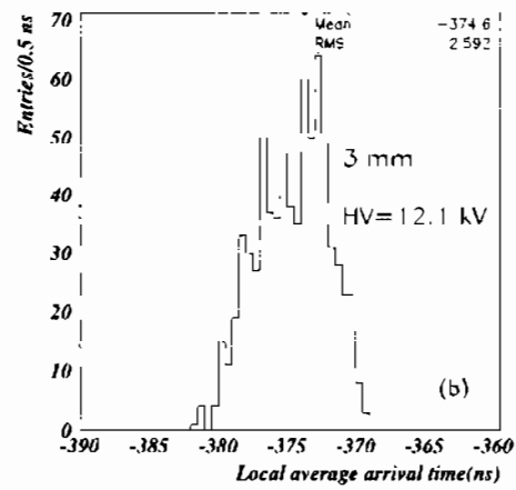
Figure 3.16: Sigmas (a) and mean values (b) of the Gaussian fits to all the local ( 1 \times 1 \text{ cm}^2 cells) time distributions for the 3 mm chamber at HV=12.1 kV.
